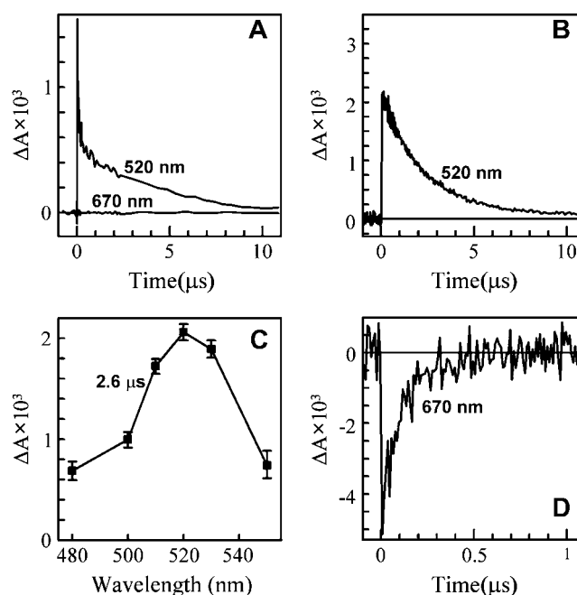
FIGURE 2 (A) Time-resolved transient absorption difference profiles probed at 520 nm and 670 nm, which represent triplet ^3\text{Car}^* and ^3\text{Chl}^* population dynamics. The b_6f complex purified via crystallization was excited at 660 nm under aerobic conditions. The amplitude of the absorbance changes at 670 nm is zero relative to the noise level. (B) Transient absorption measured at 520 nm for the conventionally purified complex under the same conditions. (C) The amplitude of the 2.6 \mu\text{s} component associated with ^3\text{Car}^* formation shown in panel B as a function of probe wavelength. (D) Transient absorption signal probed at 670 nm for the conventionally purified complex is not zero and stems from nonspecifically bound chlorophylls.
